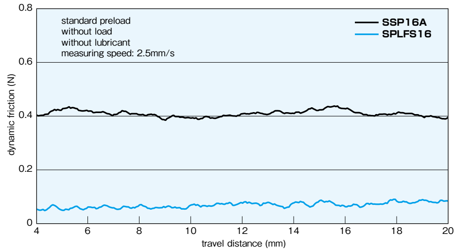
Figure B-38 Comparison of Dynamic Friction
