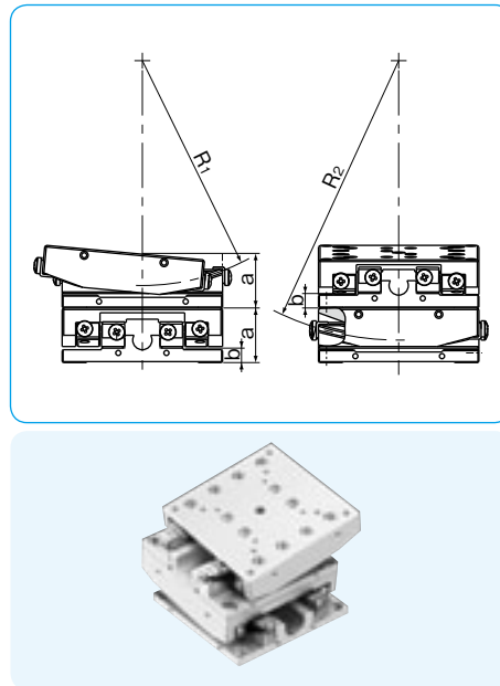
Figure G-42 Two Axes Specification
