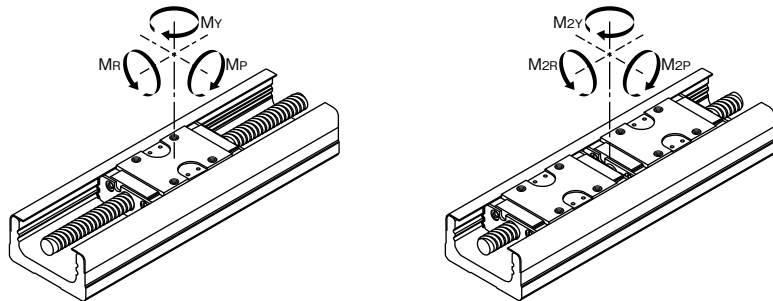
Figure H-5 Direction of Moment
