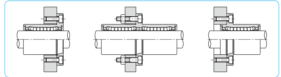
Figure C-6 Flange Type
