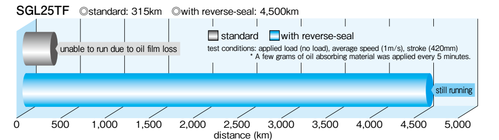
Figure A-32 Grease Dry-up Test Data
