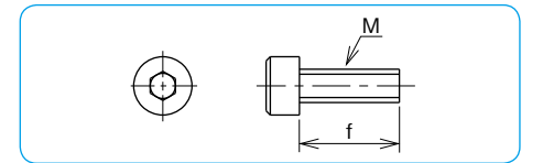
Figure A-51 Mounting Screw
