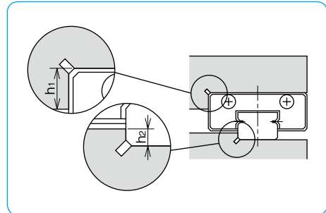
Figure A-49 Mounting Reference Surface Profile-1
