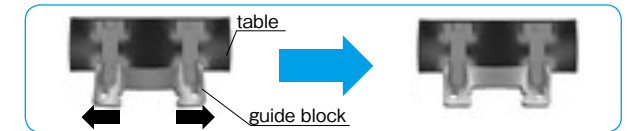
Figure A-35 SEB type AD profile
