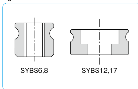
Figure G-27 Profile of SYBS Bed
